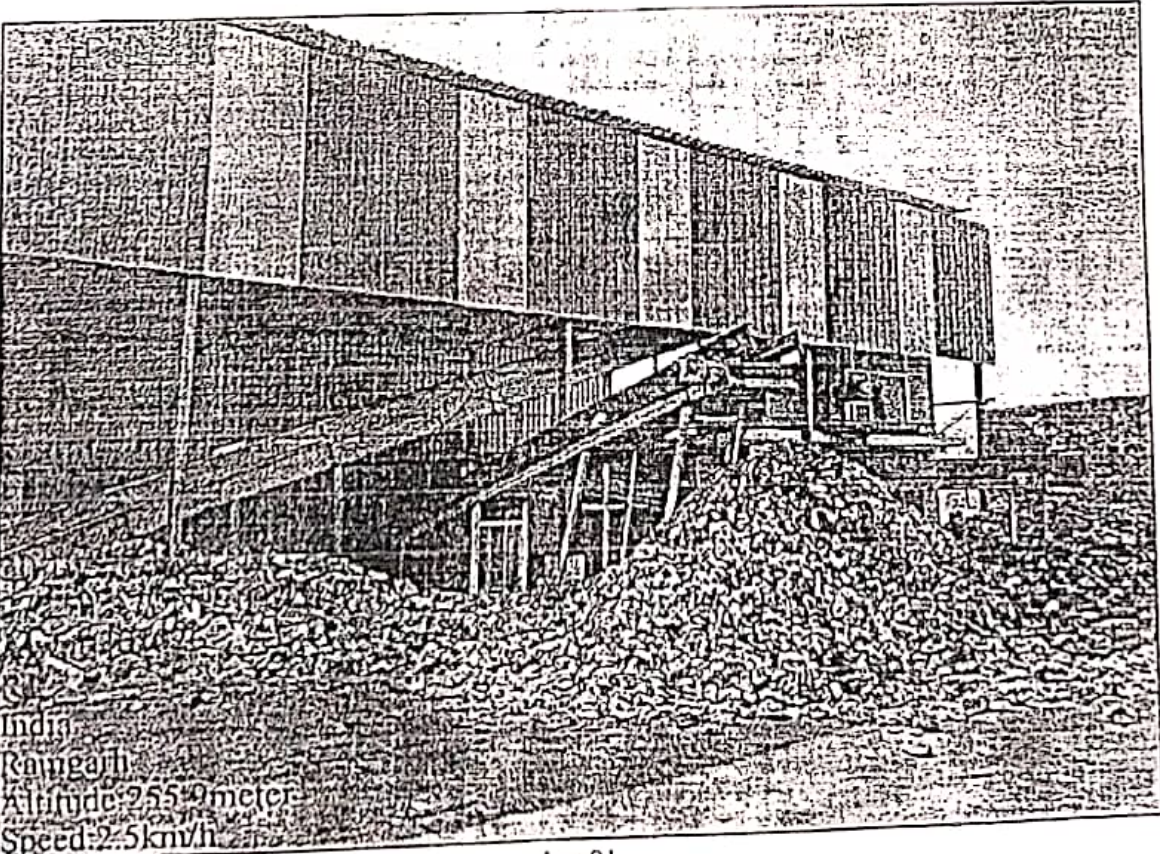
Fig 03: Non-operative ballistic separator number 01.
